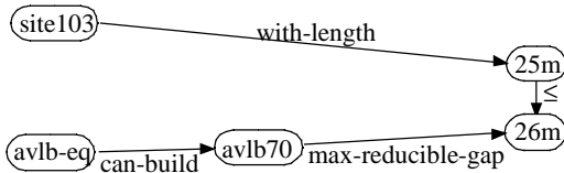
Figure 8: Guiding the agent to generate explanations.
